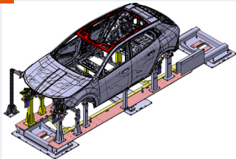
BODY-IN-WHITE FIXTURE
